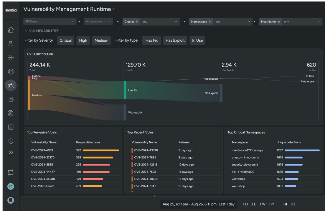
Figure 1: Runtime Vulnerability Management
