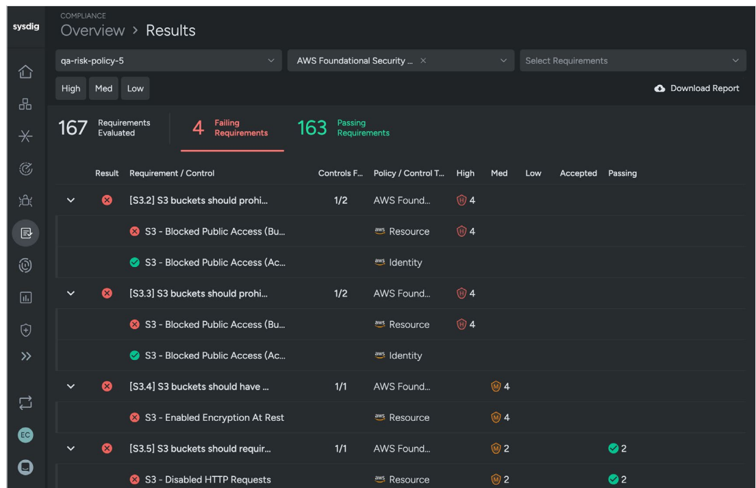
Figure 2: AWS cloud security posture report
